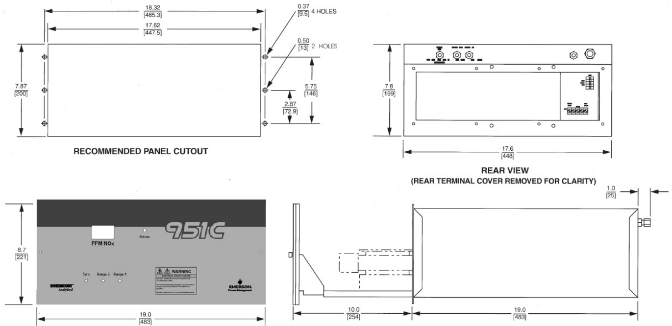
Drawing 1-1. Panel Cutout / Installation Drawing
